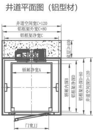
注：铝型材井道圆梁间距1200mm
